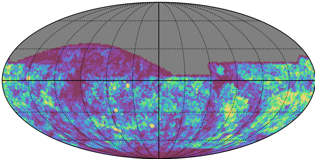
reweight_plane_v3.3_10yrs g band: Gaps_24hr
