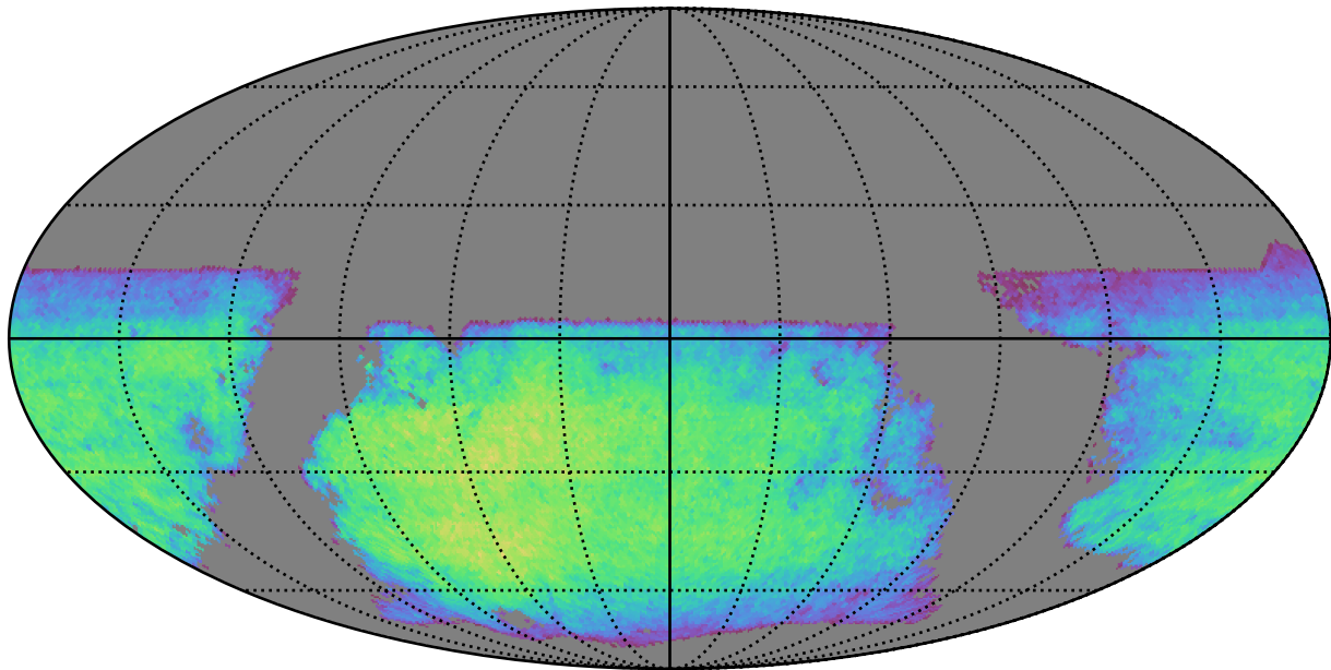
reweight_plane_v3.3_10yrs i band non-DD year 8: ExgalM5WithCuts
