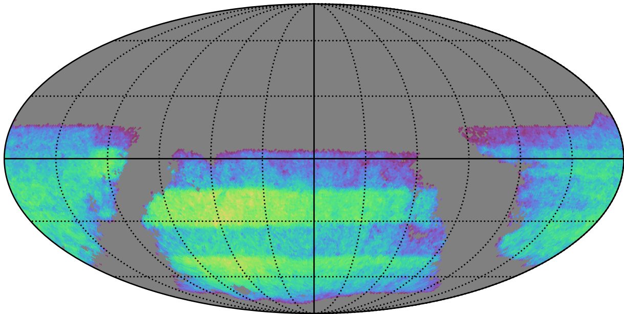
reweight_plane_v3.3_10yrs i band non-DD year 3: ExgalM5WithCuts
