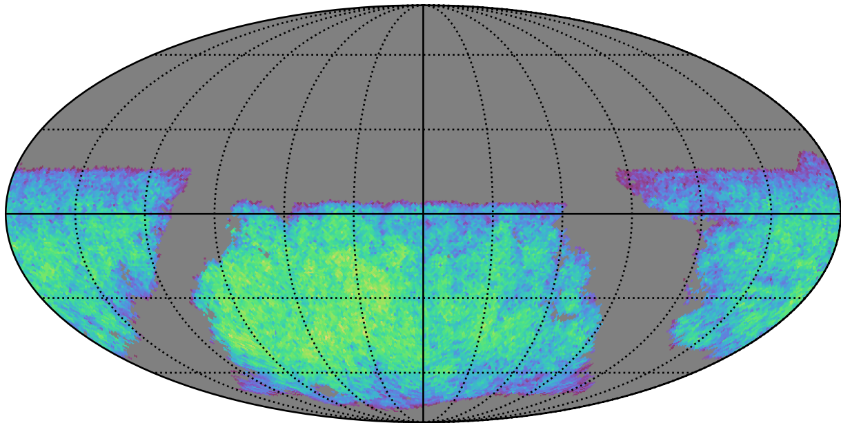
reweight_plane_v3.3_10yrs i band non-DD year 1: ExgalM5WithCuts
