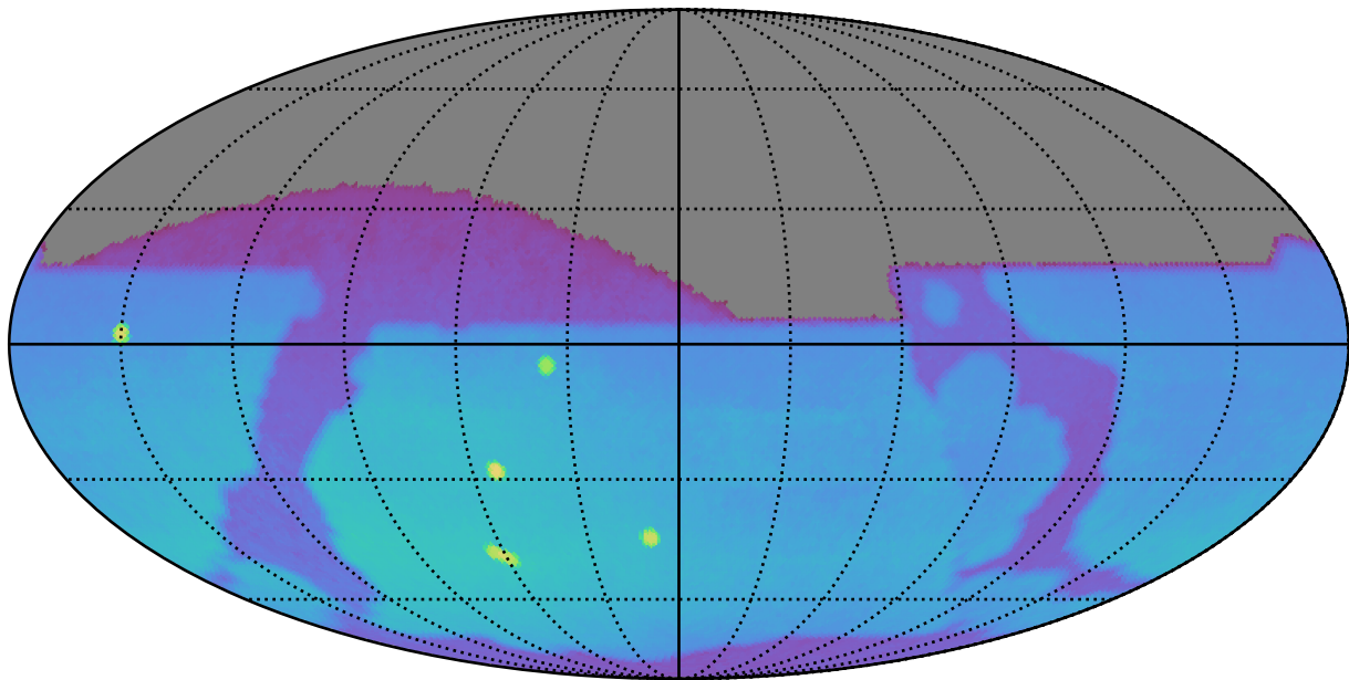
reweight_plane_v3.3_10yrs : Brown Dwarf, L7
