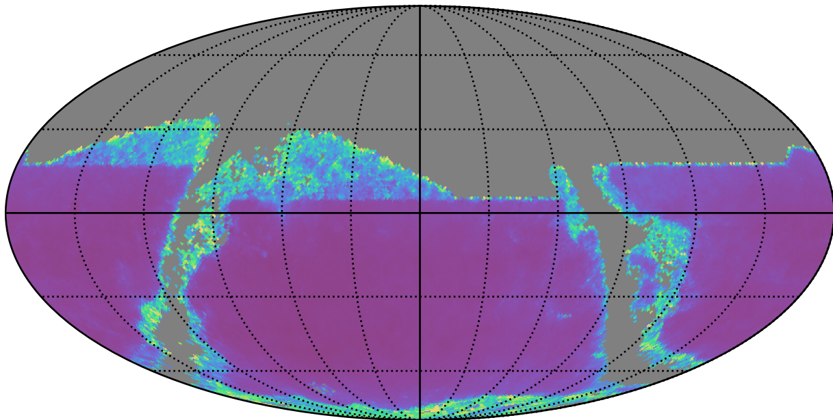
reweight_plane_v3.3_10yrs z band: AGN SF_uncert
