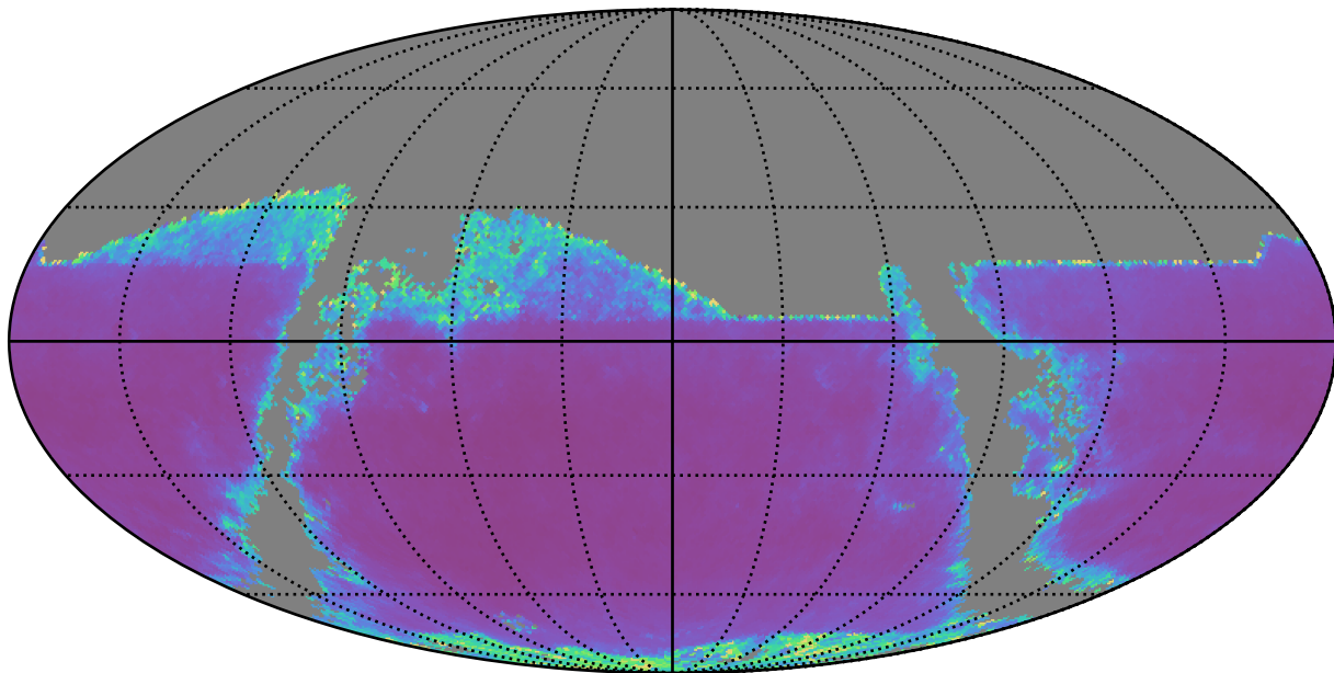
reweight_plane_v3.3_10yrs i band: AGN SF_uncert
