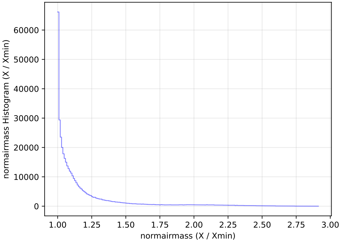
reweight_plane_v3.3_10yrs WFD z band: normairmass Histogram
