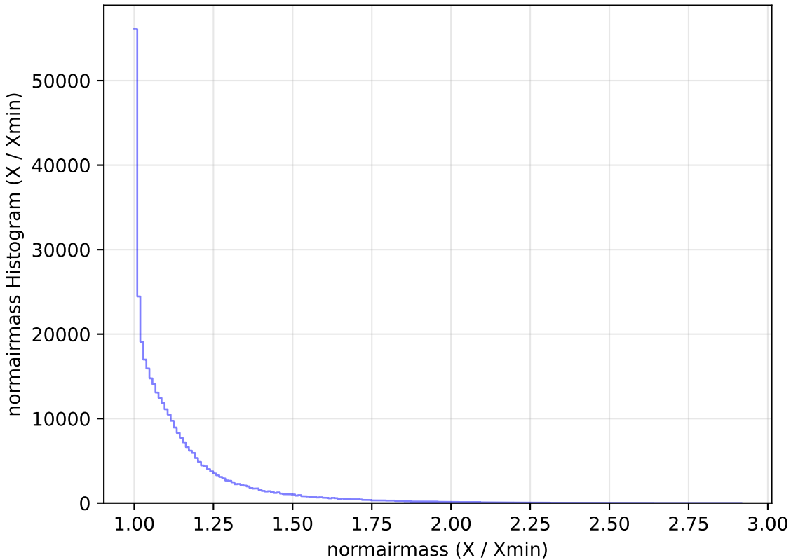
reweight_plane_v3.3_10yrs WFD y band: normairmass Histogram
