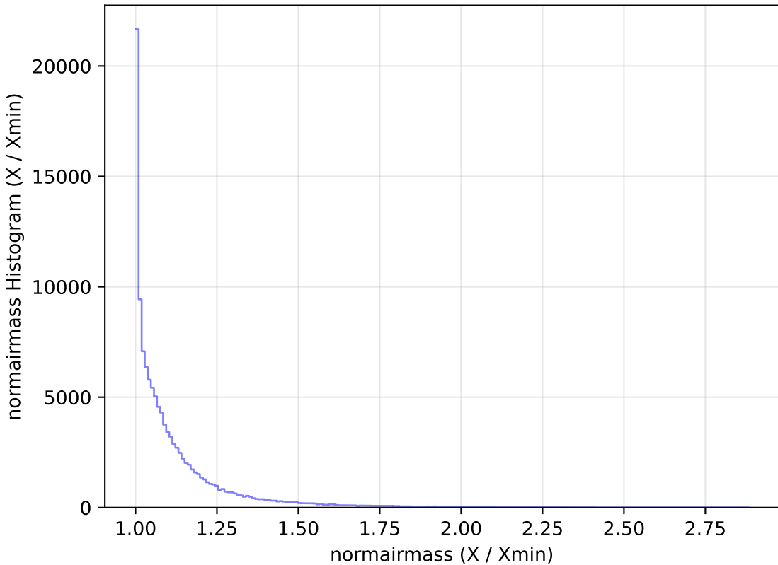
reweight_plane_v3.3_10yrs WFD u band: normairmass Histogram
