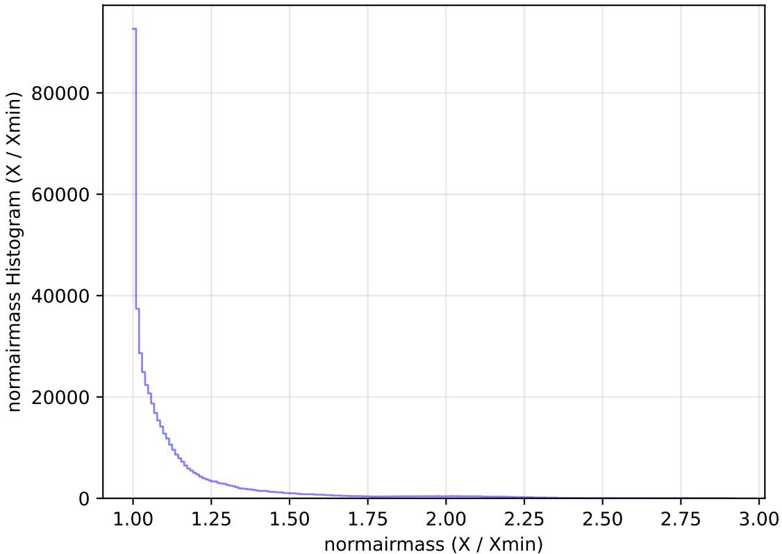
reweight_plane_v3.3_10yrs WFD r band: normairmass Histogram
