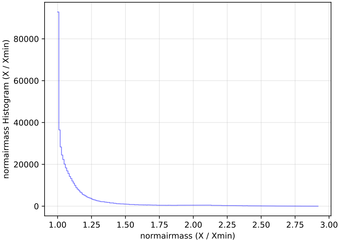
reweight_plane_v3.3_10yrs WFD i band: normairmass Histogram
