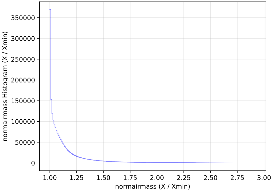
reweight_plane_v3.3_10yrs WFD all bands: normairmass Histogram
