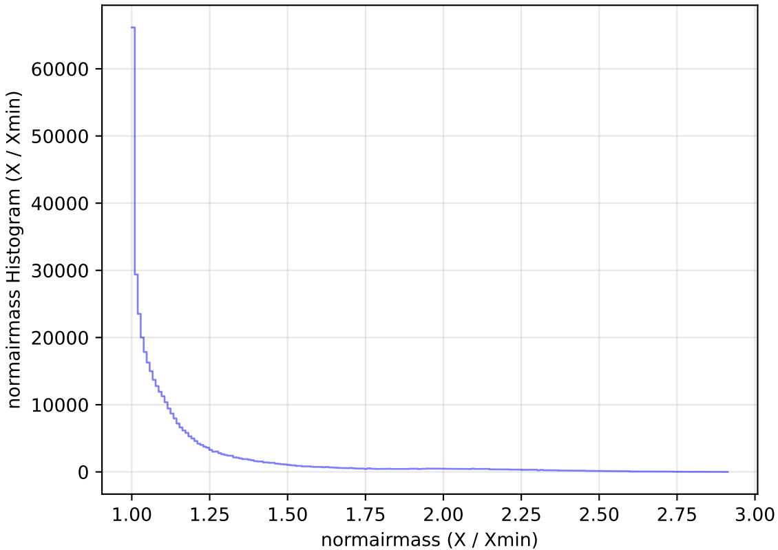
reweight_plane_v3.3_10yrs All sky z band: normairmass Histogram
