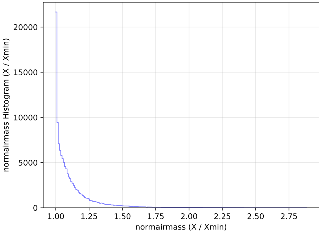
reweight_plane_v3.3_10yrs All sky u band: normairmass Histogram
