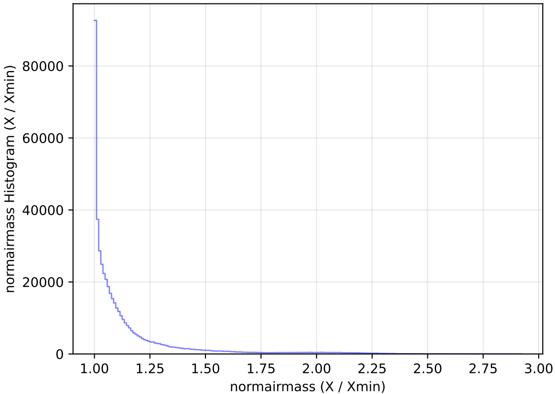
reweight_plane_v3.3_10yrs All sky r band: normairmass Histogram
