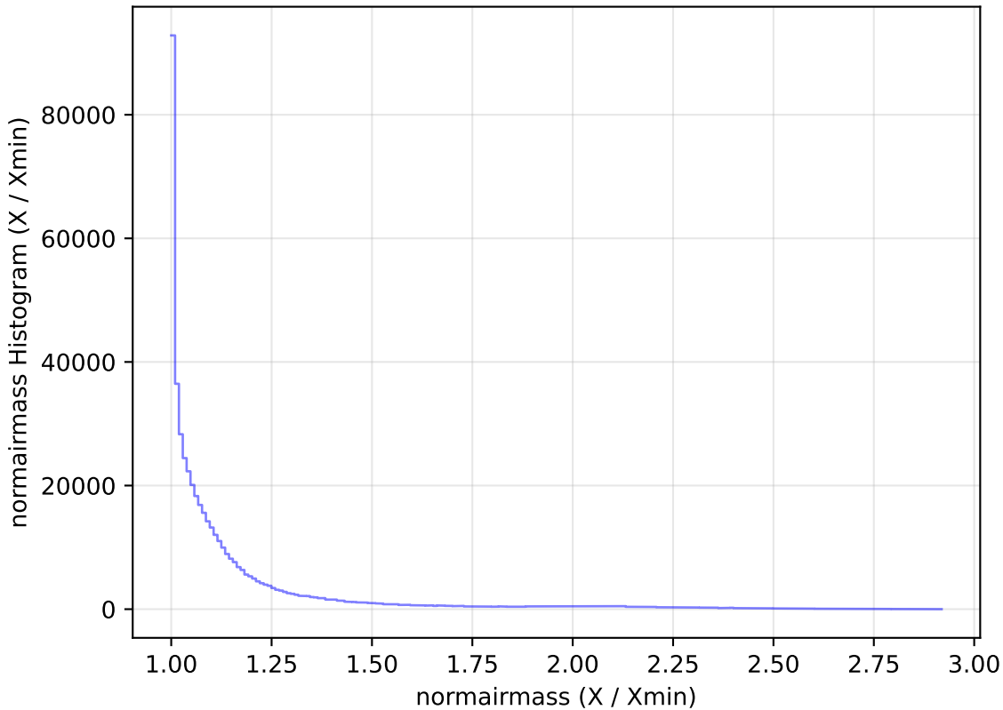
reweight_plane_v3.3_10yrs All sky i band: normairmass Histogram
