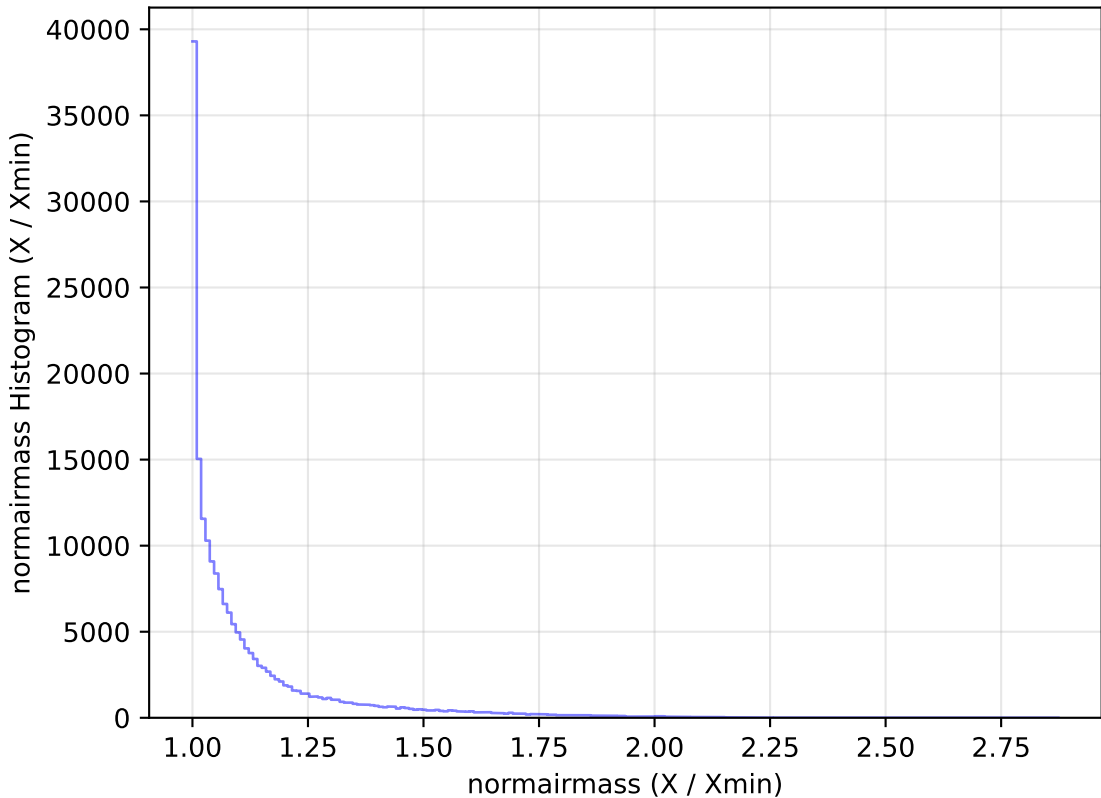
reweight_plane_v3.3_10yrs All sky g band: normairmass Histogram
