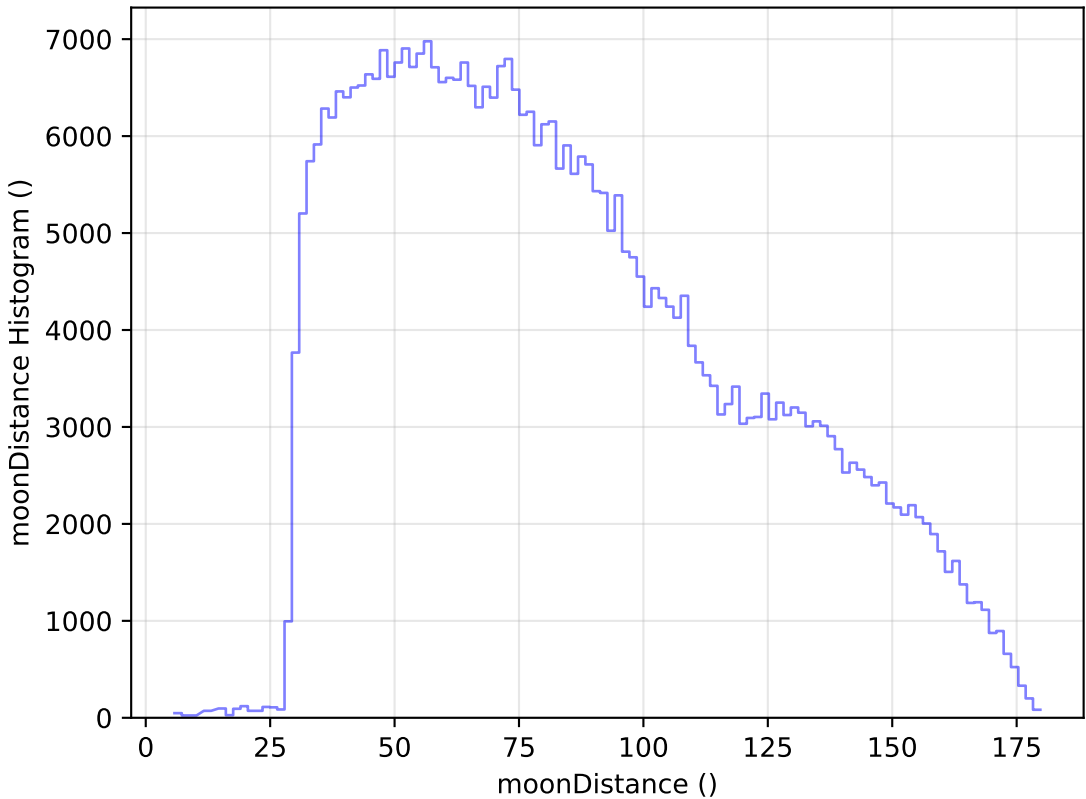
reweight_plane_v3.3_10yrs WFD z band: moonDistance Histogram
