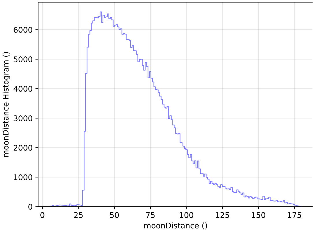
reweight_plane_v3.3_10yrs WFD y band: moonDistance Histogram
