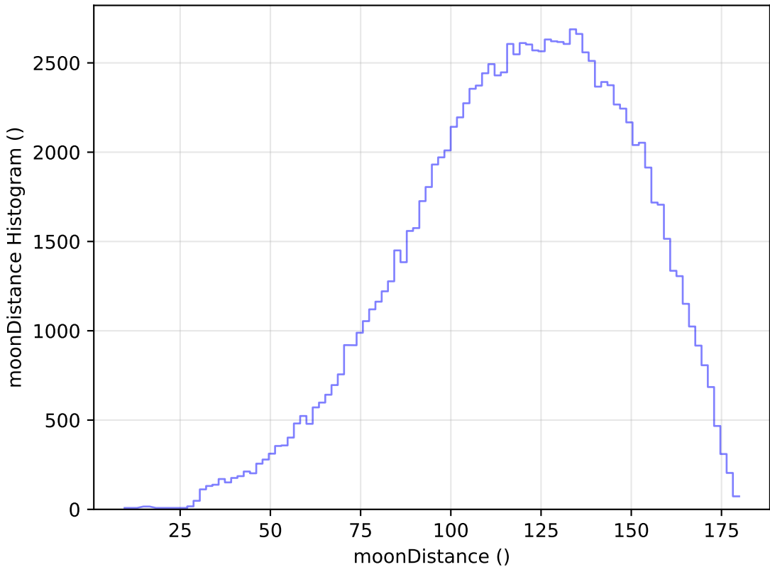
reweight_plane_v3.3_10yrs WFD u band: moonDistance Histogram
