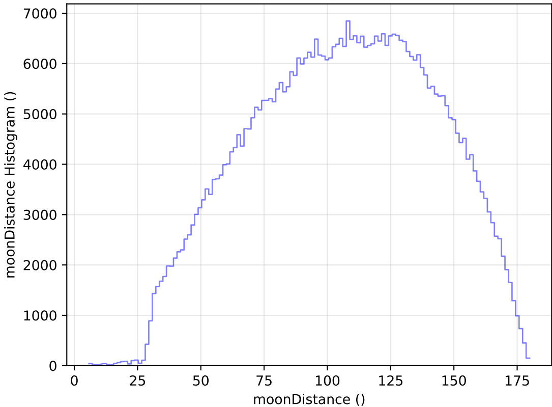
reweight_plane_v3.3_10yrs WFD r band: moonDistance Histogram
