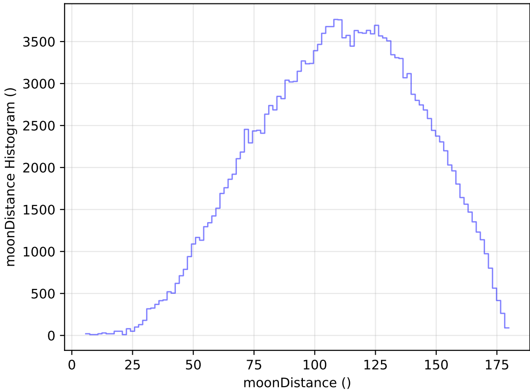
reweight_plane_v3.3_10yrs WFD g band: moonDistance Histogram
