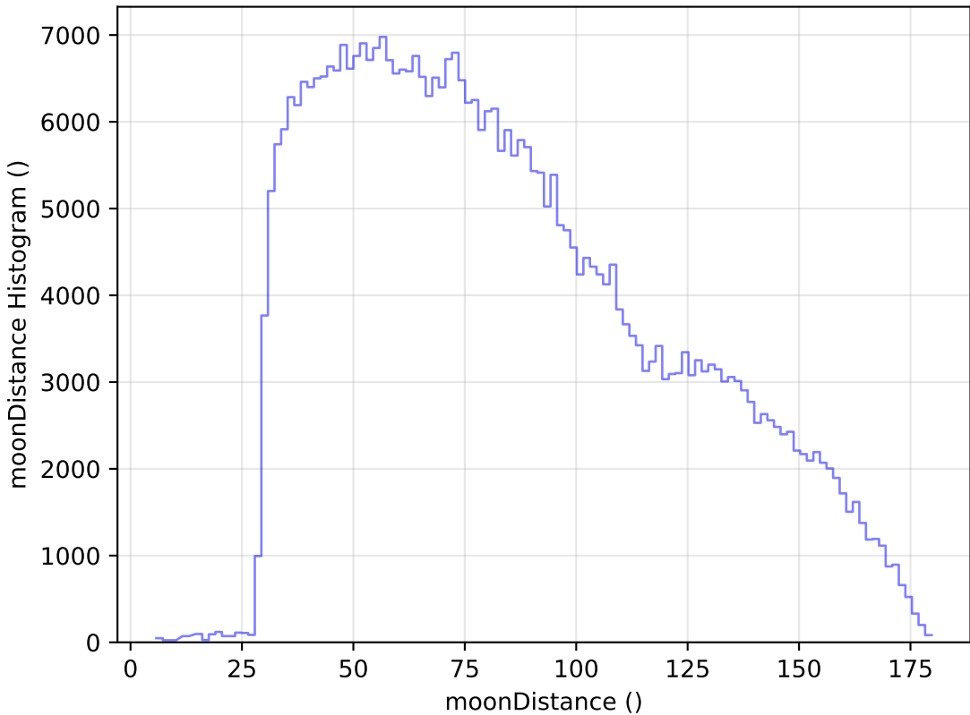
reweight_plane_v3.3_10yrs All sky z band: moonDistance Histogram
