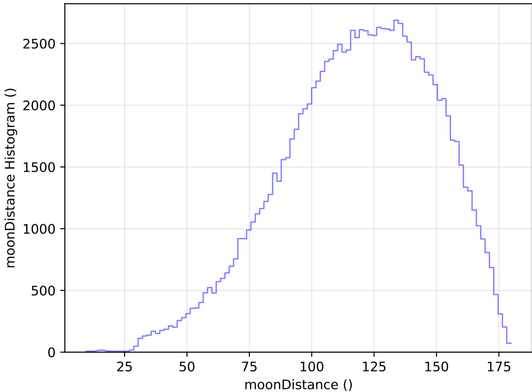
reweight_plane_v3.3_10yrs All sky u band: moonDistance Histogram
