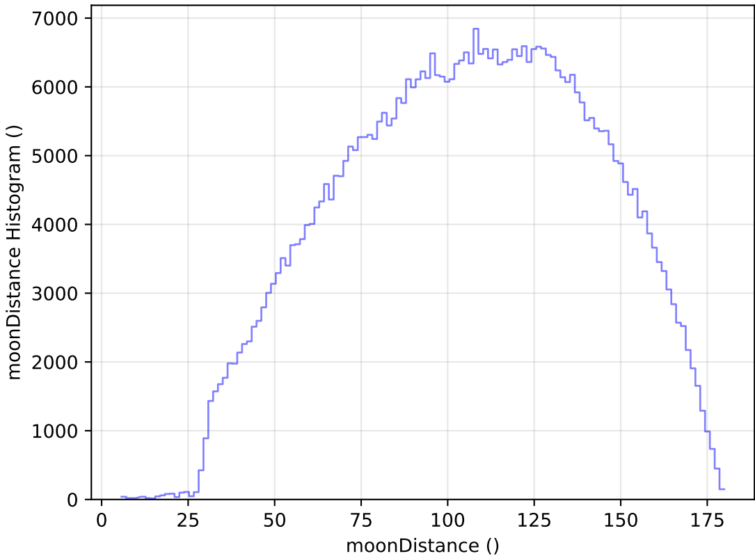
reweight_plane_v3.3_10yrs All sky r band: moonDistance Histogram
