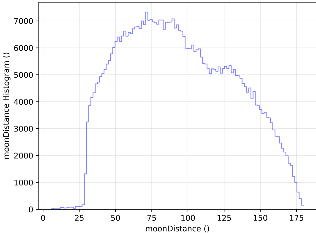
reweight_plane_v3.3_10yrs All sky i band: moonDistance Histogram
