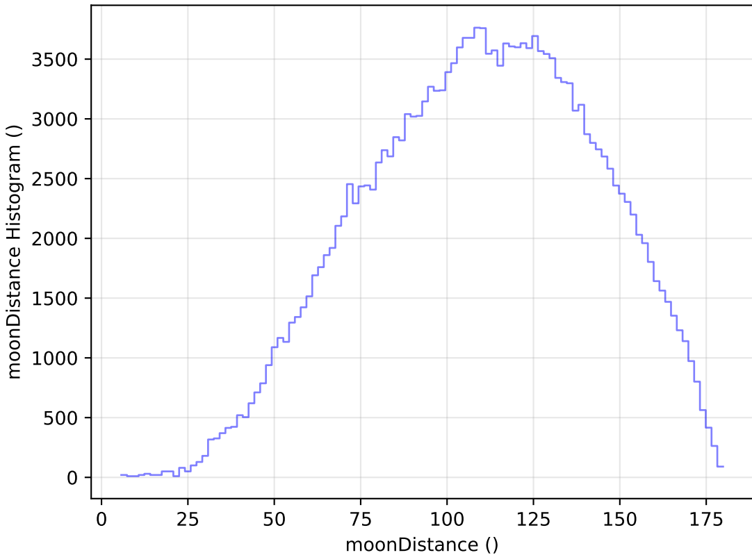
reweight_plane_v3.3_10yrs All sky g band: moonDistance Histogram
