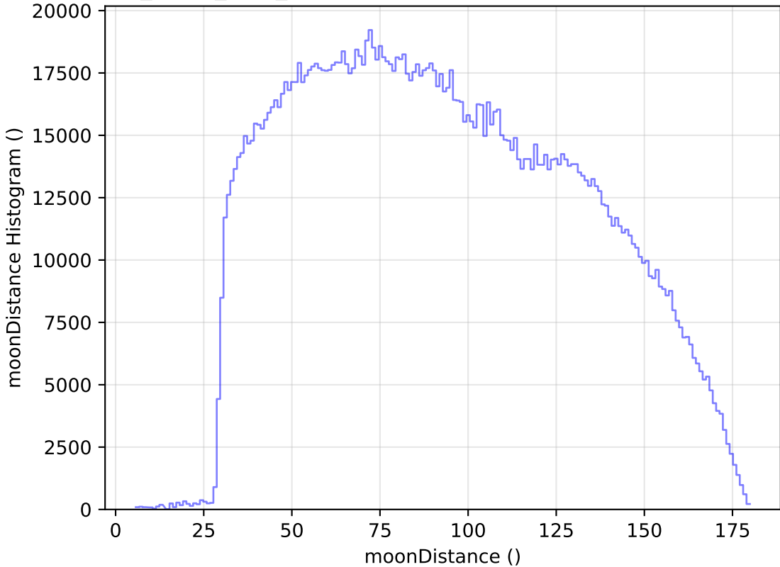
reweight_plane_v3.3_10yrs All sky all bands: moonDistance Histogram
