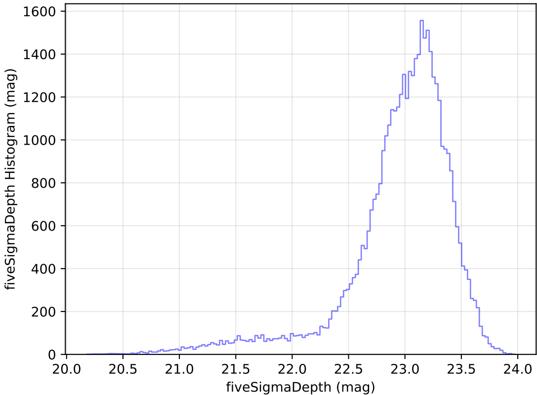
reweight_plane_v3.3_10yrs Yr 1 z band: fiveSigmaDepth Histogram
