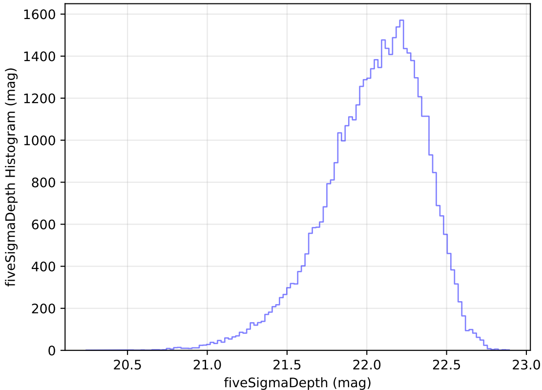
reweight_plane_v3.3_10yrs Yr 1 y band: fiveSigmaDepth Histogram
