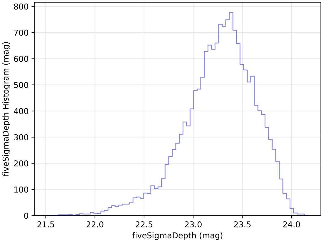
reweight_plane_v3.3_10yrs Yr 1 u band: fiveSigmaDepth Histogram
