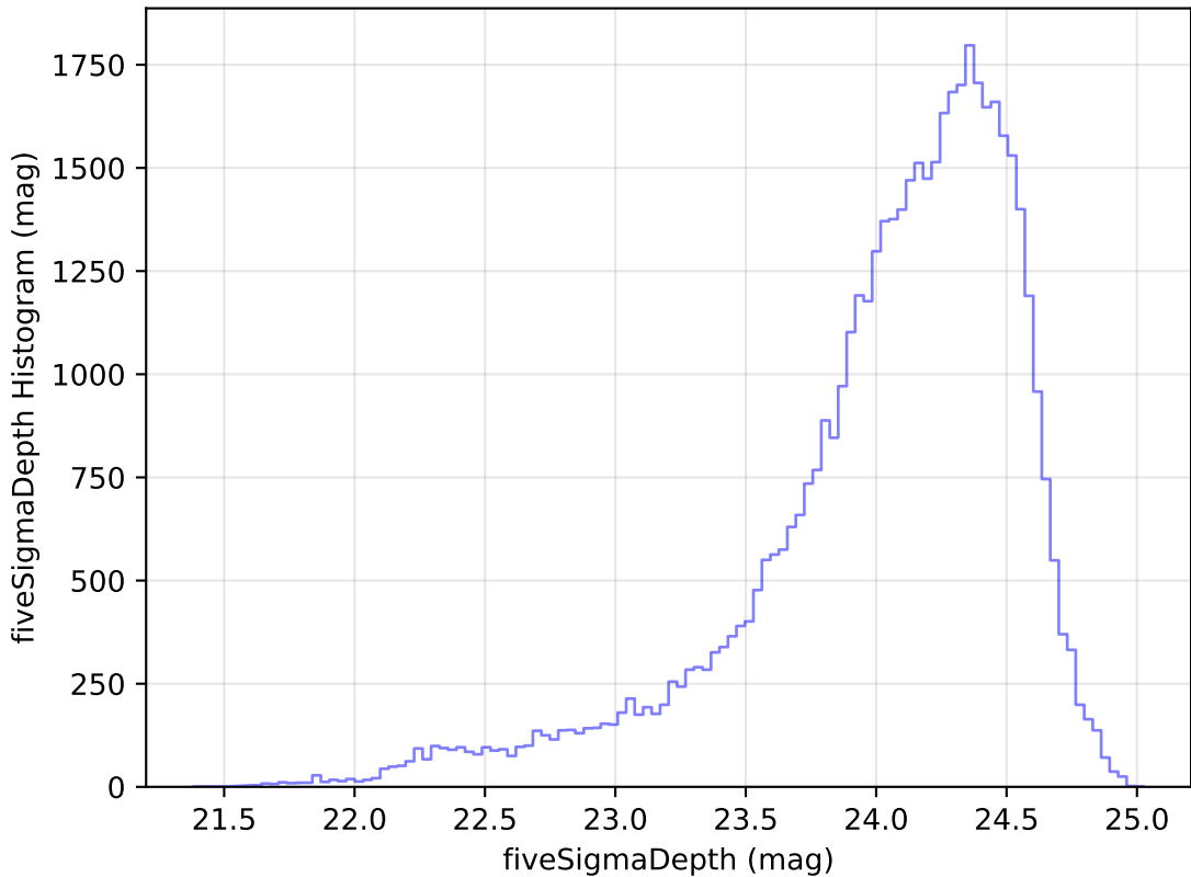
reweight_plane_v3.3_10yrs Yr 1 r band: fiveSigmaDepth Histogram
