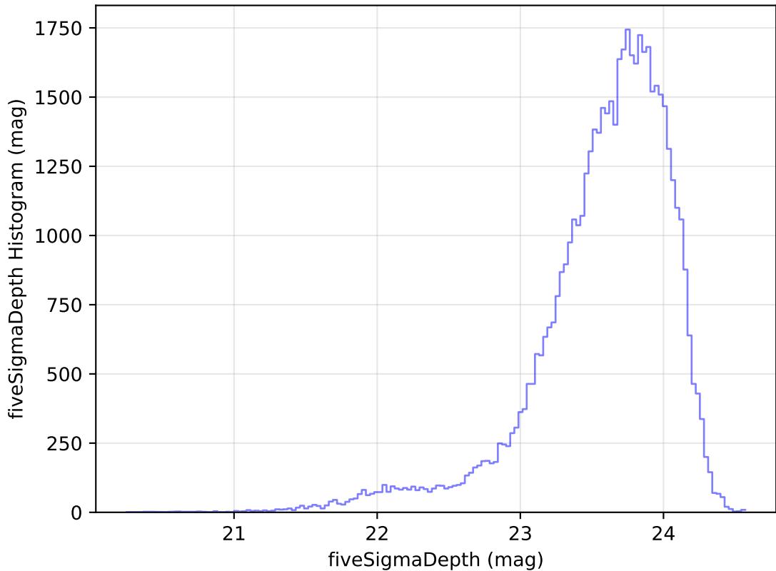
reweight_plane_v3.3_10yrs Yr 1 i band: fiveSigmaDepth Histogram
