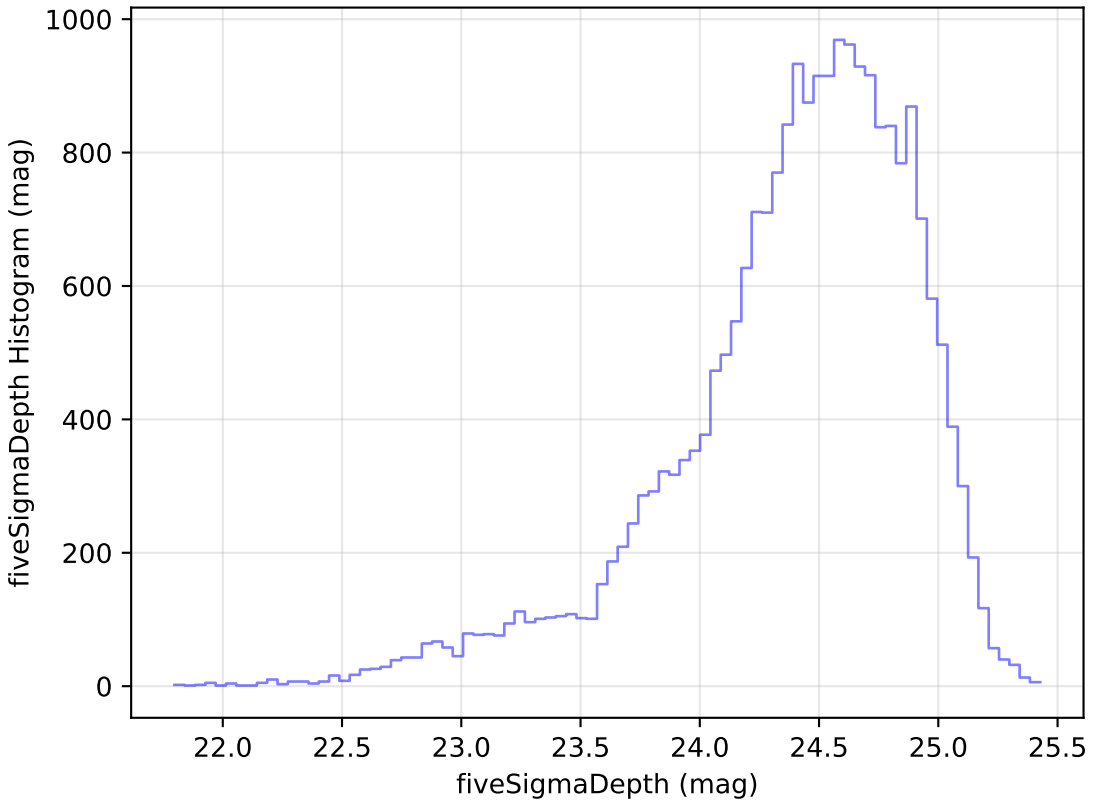
reweight_plane_v3.3_10yrs Yr 1 g band: fiveSigmaDepth Histogram
