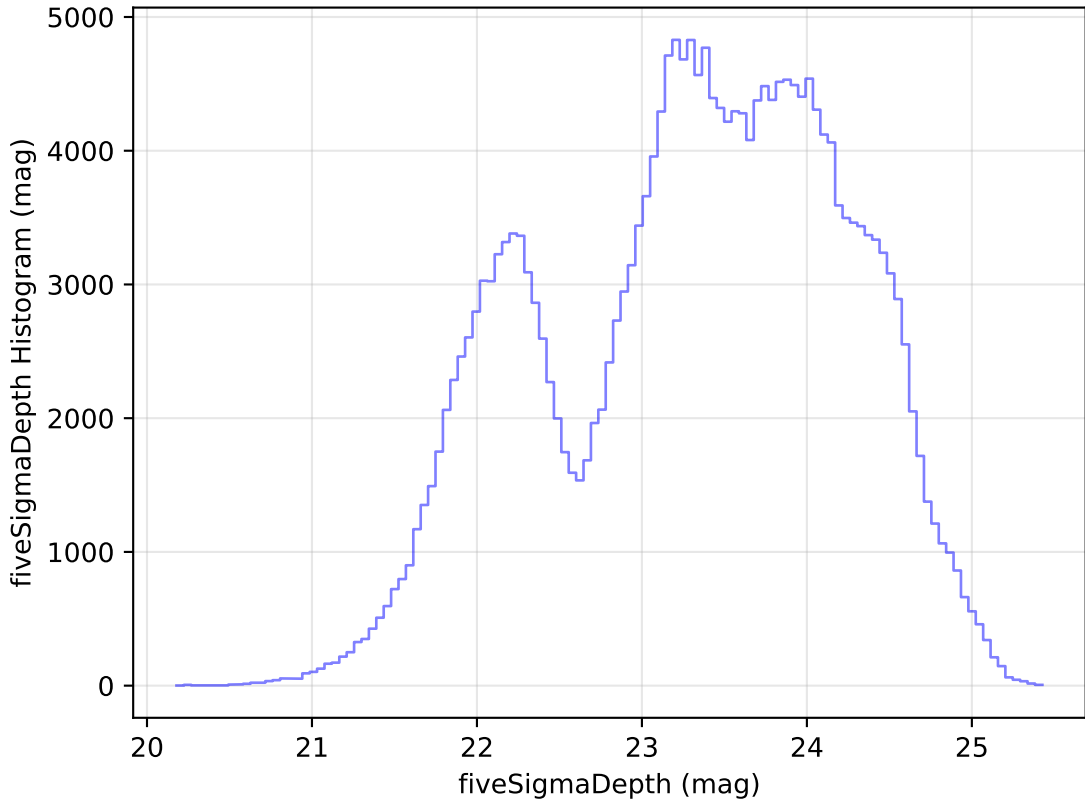
reweight_plane_v3.3_10yrs Yr 1 all bands: fiveSigmaDepth Histogram
