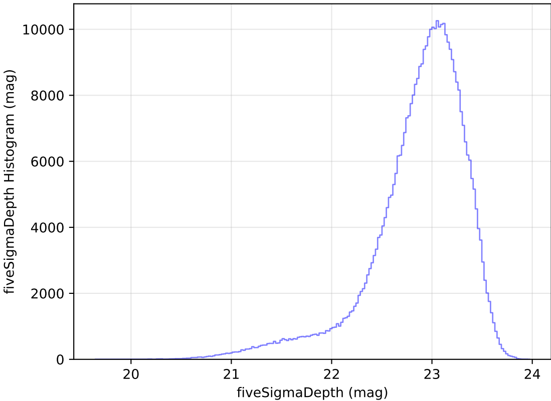
reweight_plane_v3.3_10yrs WFD z band: fiveSigmaDepth Histogram
