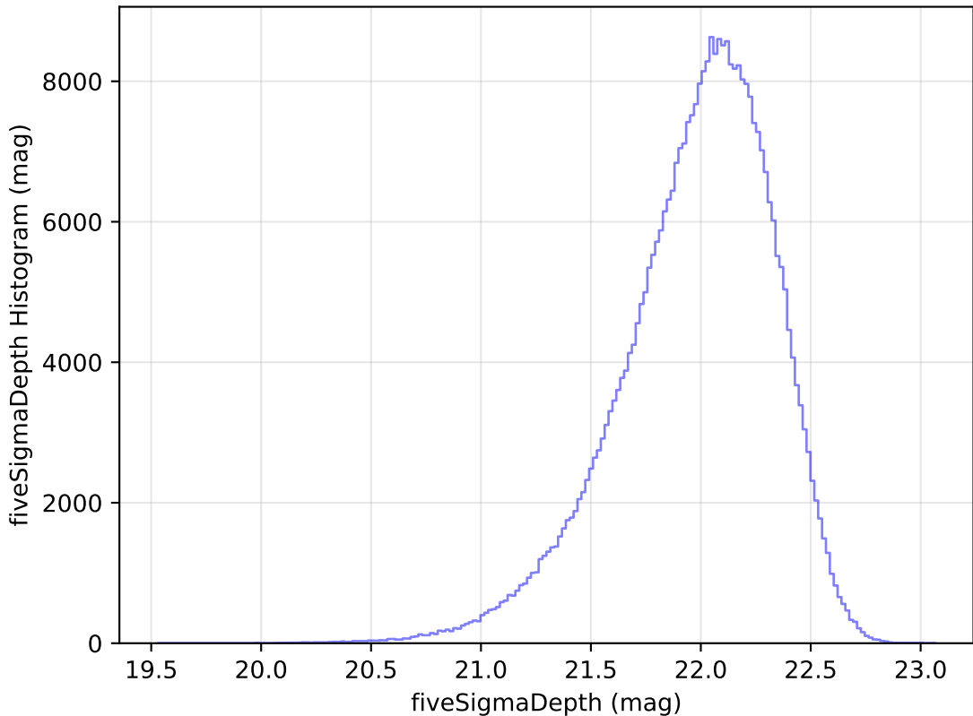
reweight_plane_v3.3_10yrs WFD y band: fiveSigmaDepth Histogram
