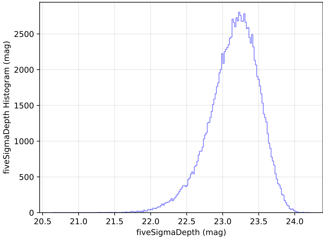
reweight_plane_v3.3_10yrs WFD u band: fiveSigmaDepth Histogram
