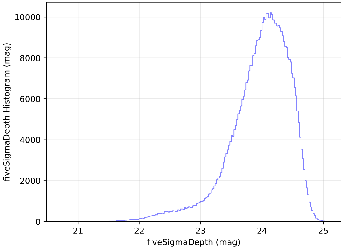
reweight_plane_v3.3_10yrs WFD r band: fiveSigmaDepth Histogram
