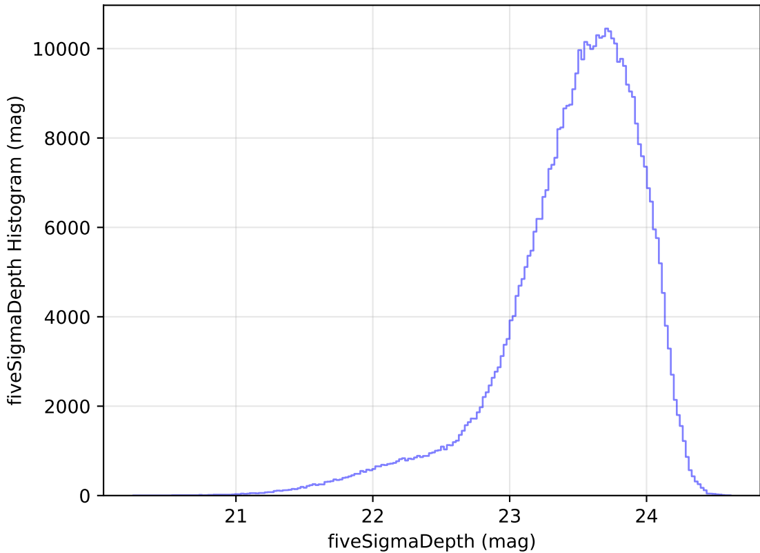
reweight_plane_v3.3_10yrs WFD i band: fiveSigmaDepth Histogram
