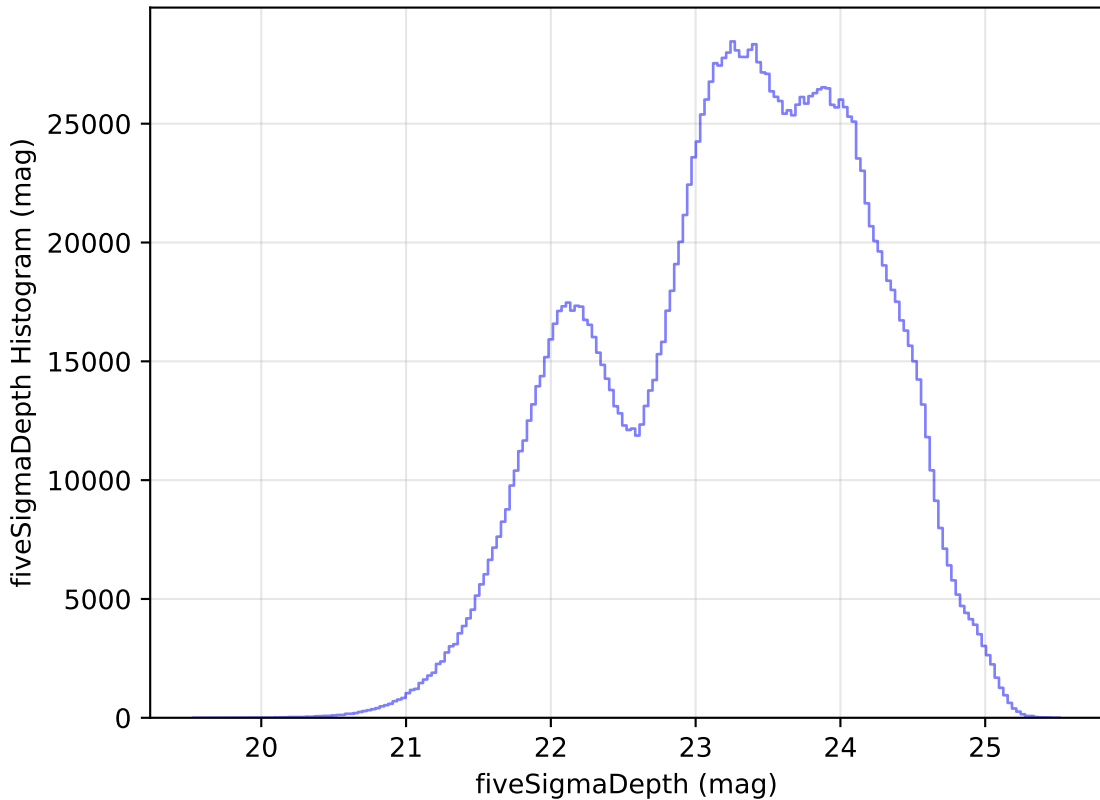
reweight_plane_v3.3_10yrs WFD all bands: fiveSigmaDepth Histogram
