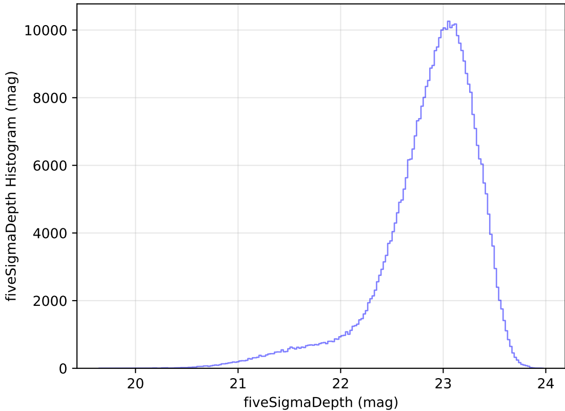
reweight_plane_v3.3_10yrs All sky z band: fiveSigmaDepth Histogram
