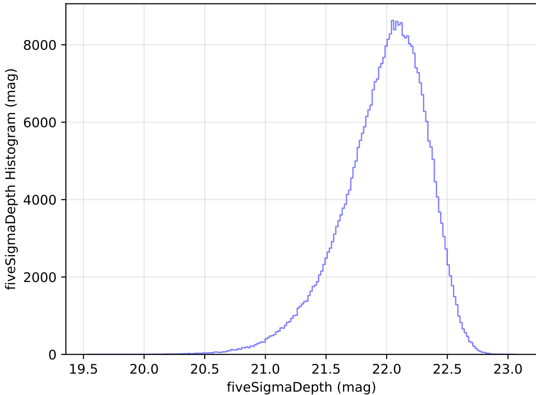
reweight_plane_v3.3_10yrs All sky y band: fiveSigmaDepth Histogram
