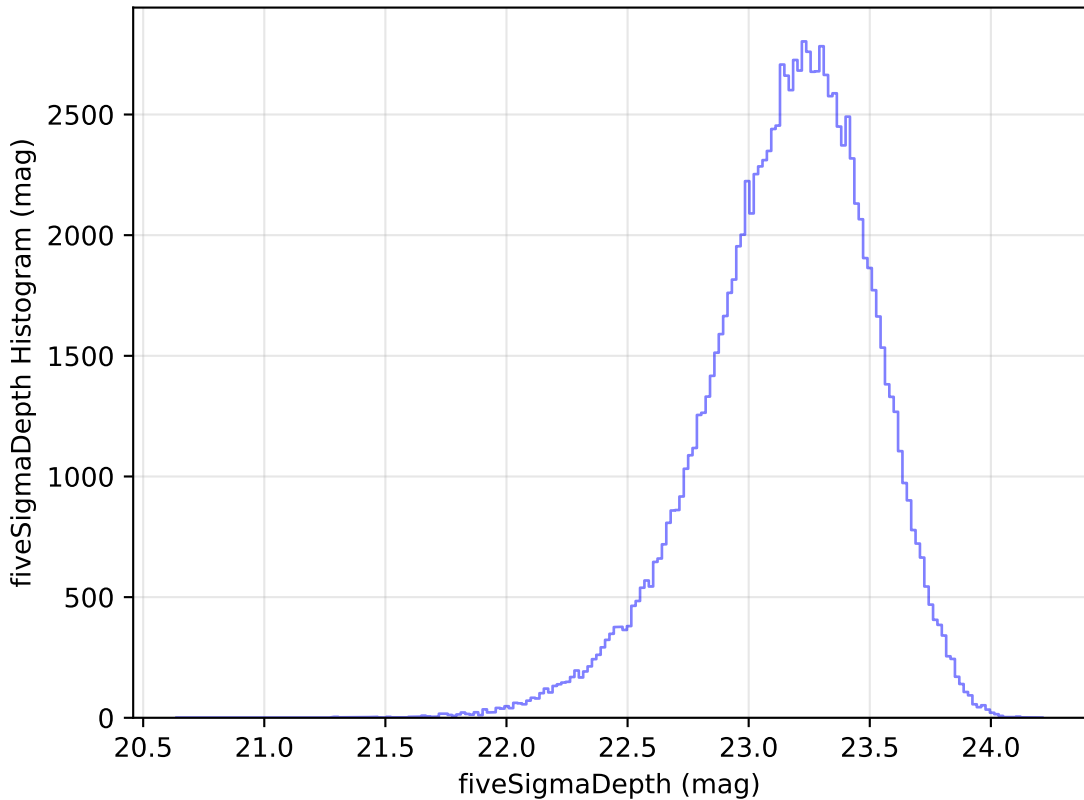
reweight_plane_v3.3_10yrs All sky u band: fiveSigmaDepth Histogram
