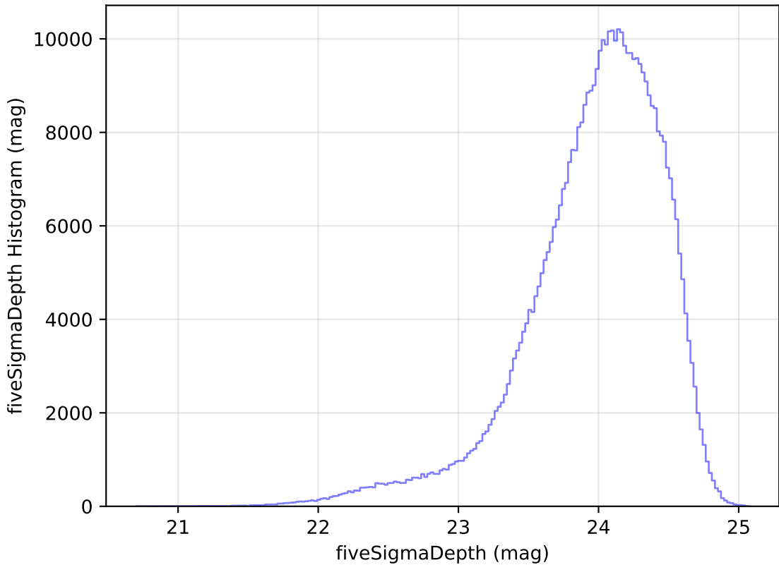
reweight_plane_v3.3_10yrs All sky r band: fiveSigmaDepth Histogram
