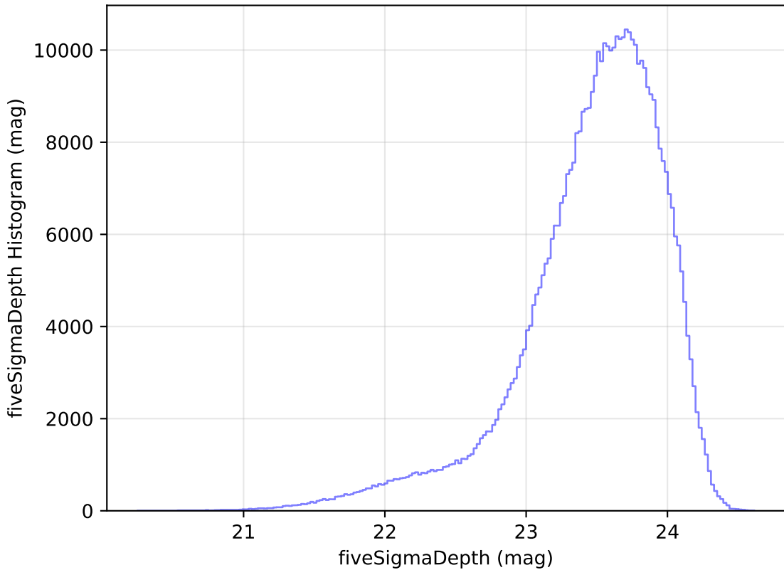
reweight_plane_v3.3_10yrs All sky i band: fiveSigmaDepth Histogram
