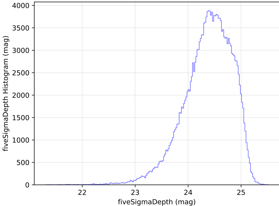
reweight_plane_v3.3_10yrs All sky g band: fiveSigmaDepth Histogram
