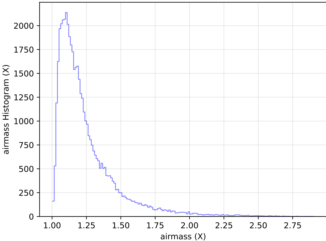
reweight_plane_v3.3_10yrs Yr 1 y band: airmass Histogram
