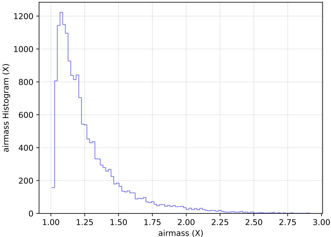
reweight_plane_v3.3_10yrs Yr 1 u band: airmass Histogram
